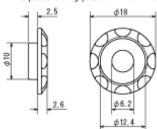
Spacer type11 (mm)
