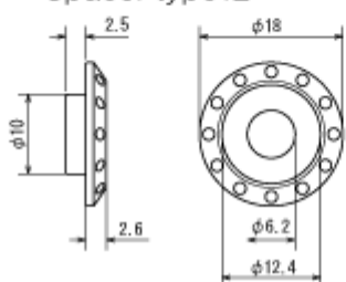
Spacer type12 (mm)
